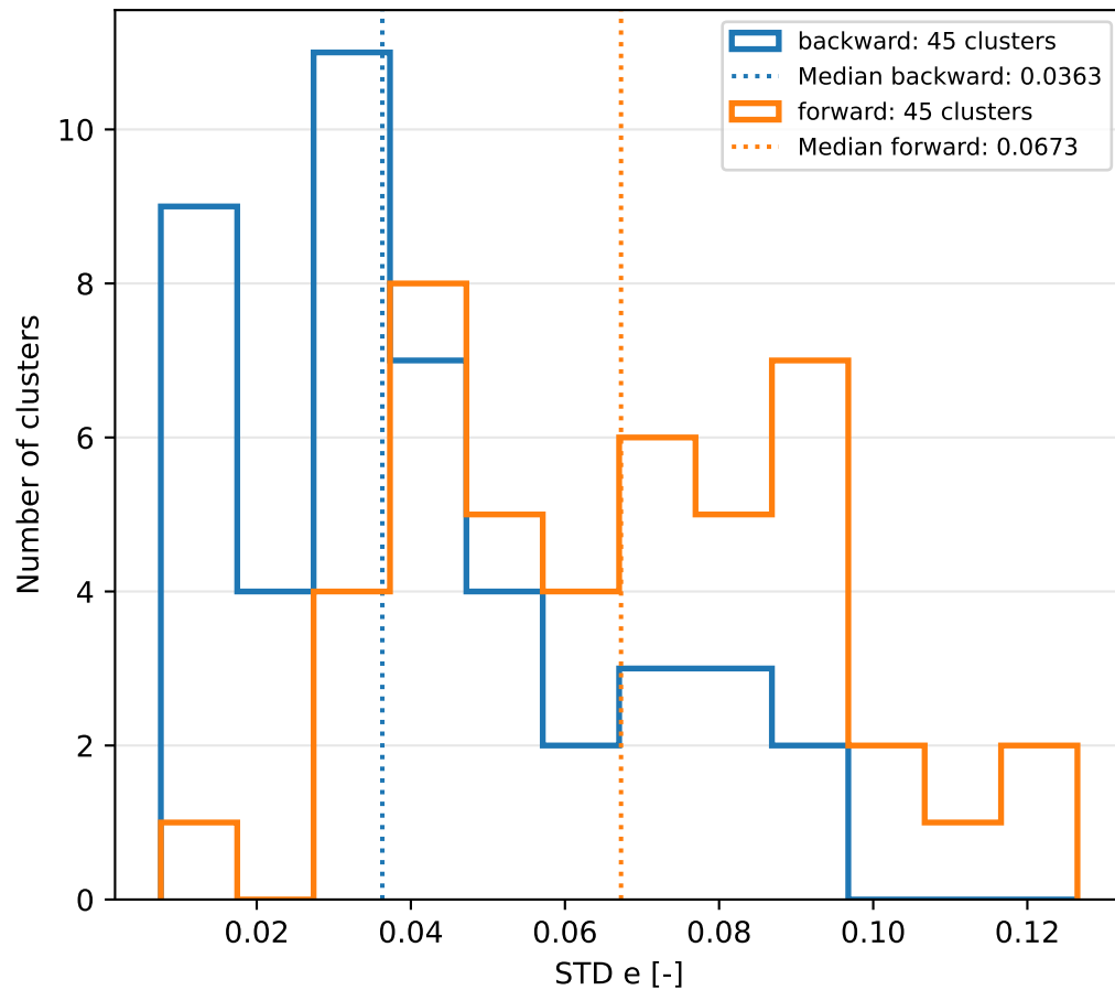
K=45 | Within-cluster STD distributions | Each cluster counts once
